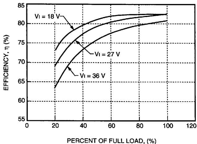
Figure 14. CC025ACL Typical Converter Efficiency
