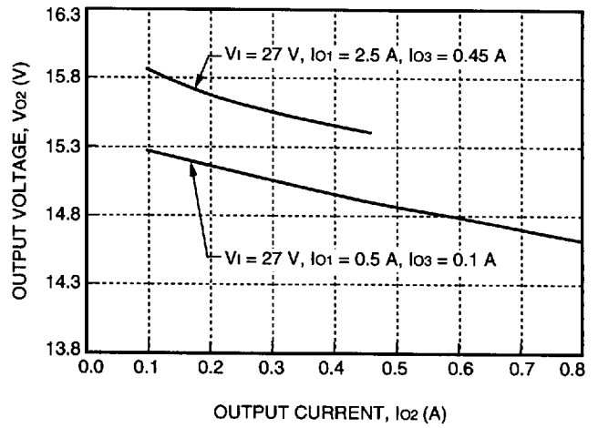
Figure 7. CC025ACL Typical Load Regulation
