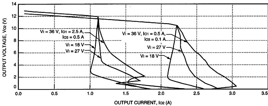
Figure 10. CC025ABK Typical 12 V Output Characteristics
