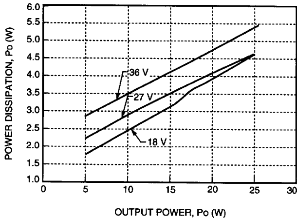
Figure 23. CC025ABK Fixed Losses, Pp
