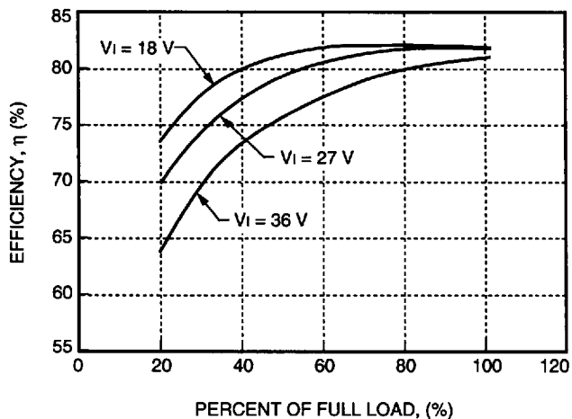
Figure 12. CC025ACL Typical 15 V Output Characteristics
