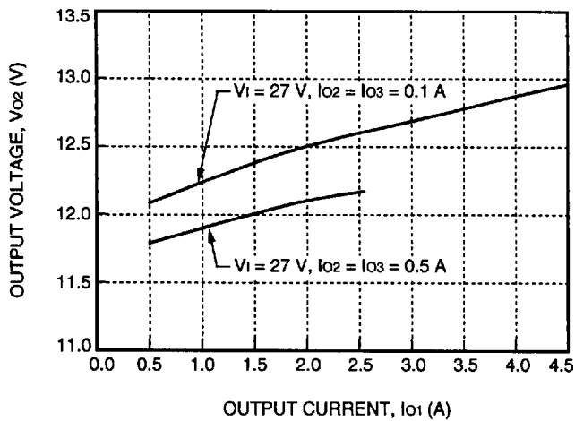
Figure 6. CC025ABK Typical Cross Regulation with Respect to I_{01}
