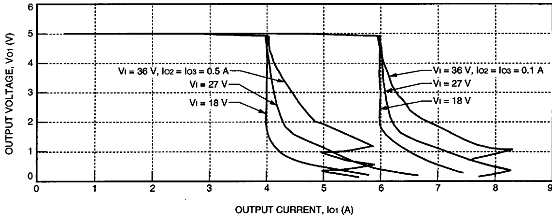
Figure 9. CC025ABK Typical 5 V Output Characteristics
