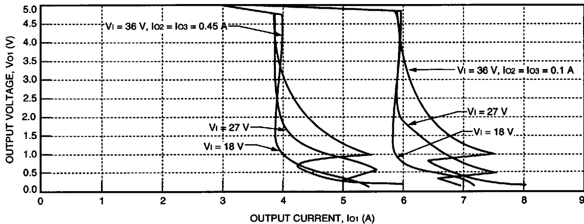
Figure 11. CC025ACL Typical 5 V Output Characteristics
