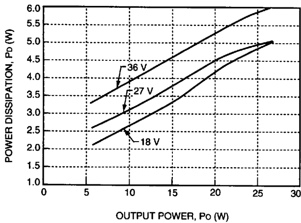
Figure 24. CC025ACL Fixed Losses, Pp
