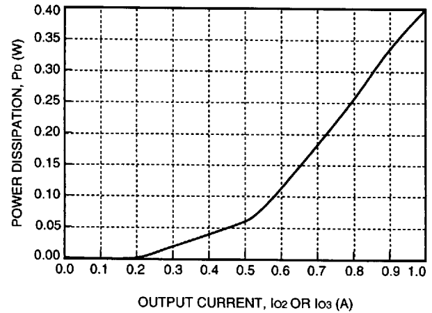
Figure 26. CC025ABK, Losses Associated with ±12 V Output, Ps2/Ps3
