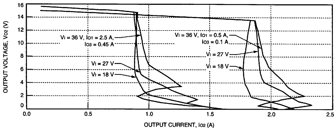
Figure 12. CC025ACL Typical 15 V Output Characteristics
