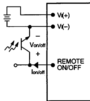
Figure 21. Remote On/Off Implementation
