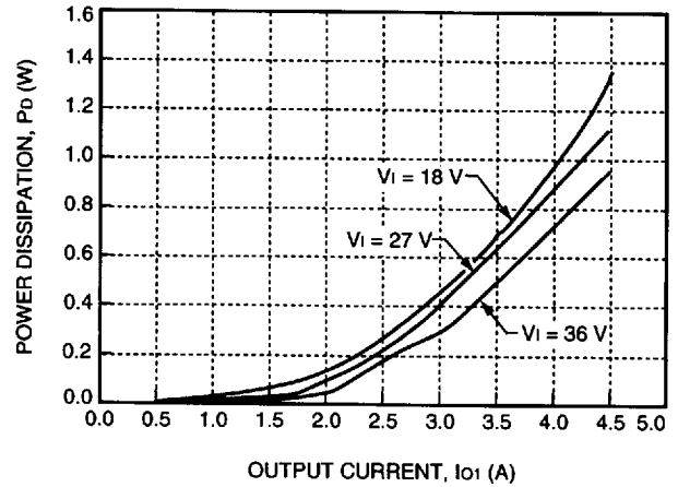
Figure 25. CC025ABK, CC025ACL Losses, Associated with 5 V Output, Ps1
