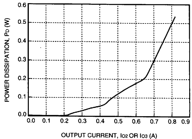
Figure 27. CC025ACL Losses Associated with ±15 V Output, Ps2/Ps3
