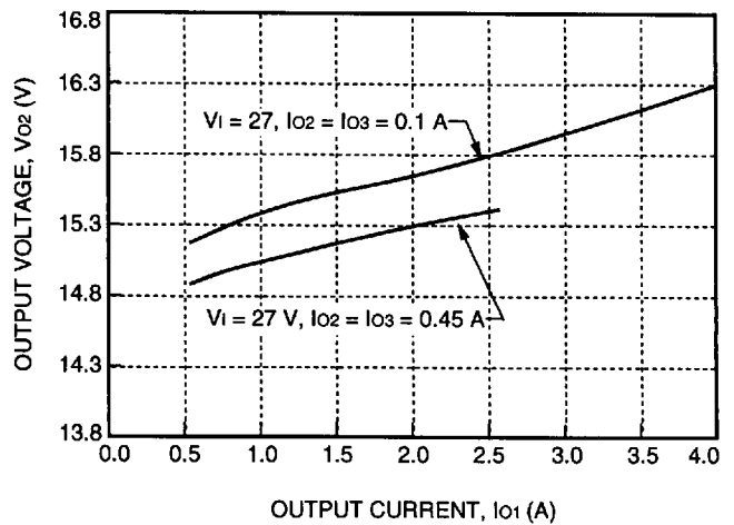
Figure 8. CC025ACL Typical Cross Regulation with Respect to I_{01}
