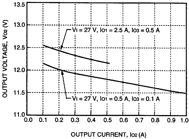
Figure 5. CC025ABK Typical Load Regulation
